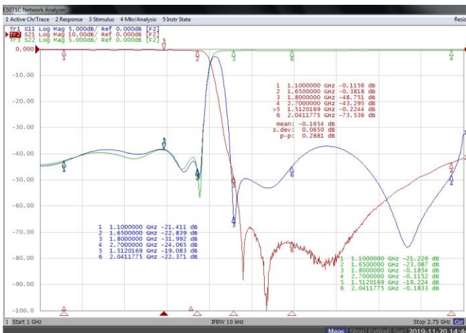
< Insertion Loss / Return Loss measurement >
